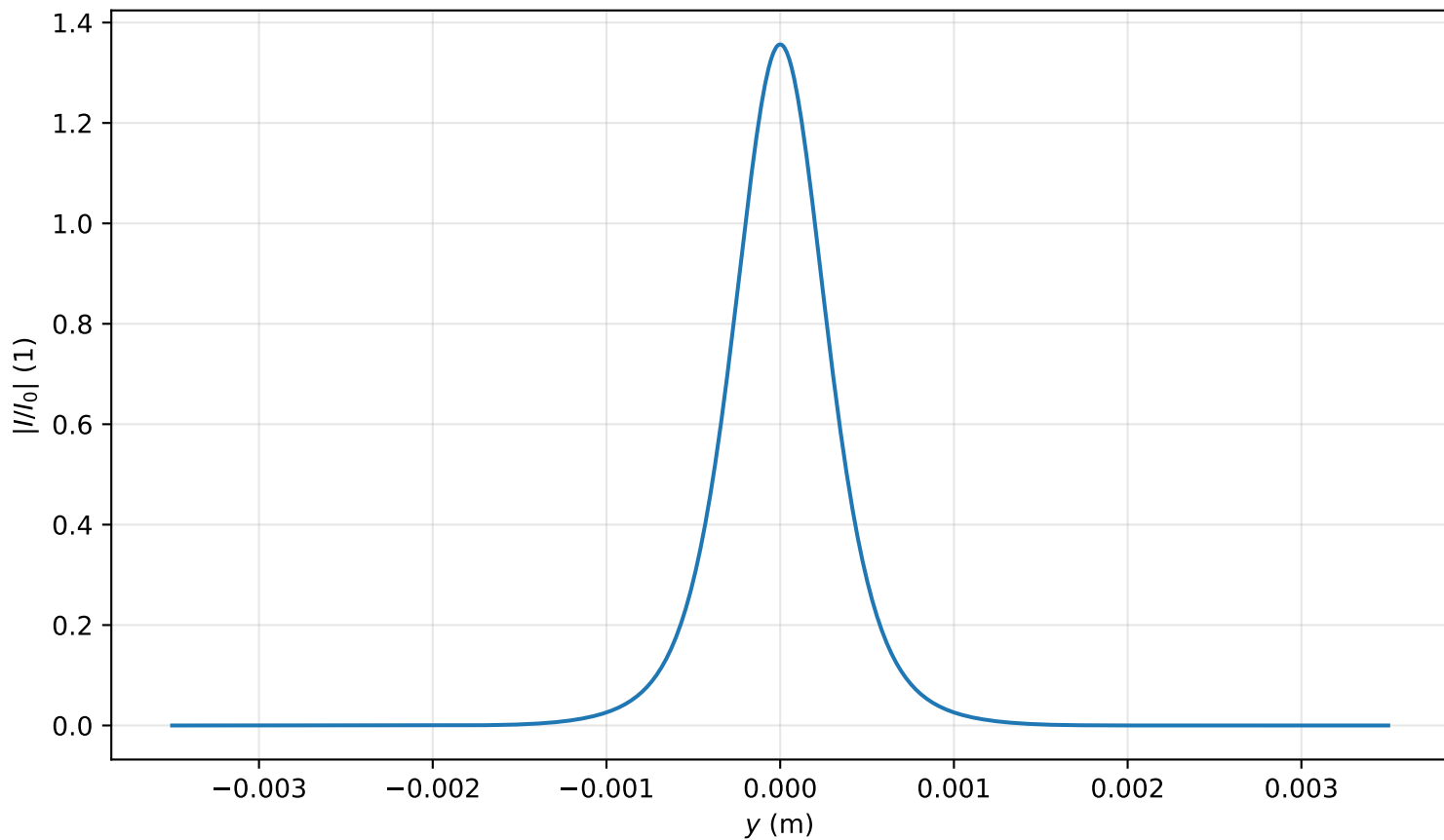
Intensity profile I(x=0, y, z=1.592)/I_0 , P_{in}=0.8P_{cr} , artificial time
